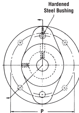
Shear Pin Assembly Dimensions (Inches)
