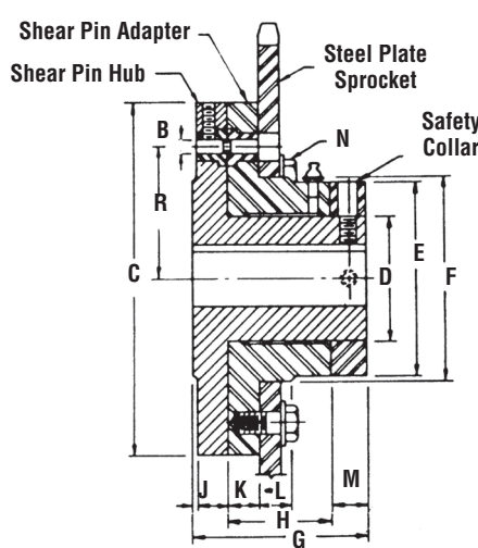
Shear Pin Assembly Dimensions (Inches)
